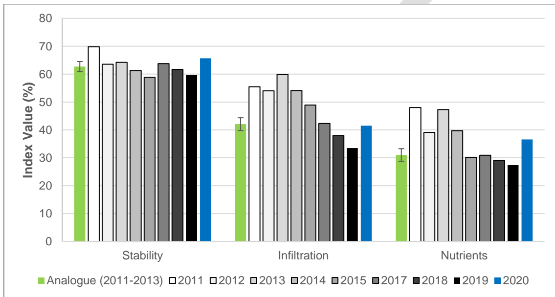
Figure 7. Landscape function indices change (2011-2020) for KANODO5 with respect to mean analogue site values (2011-2013).
